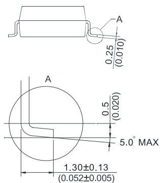
First Angle Projection
